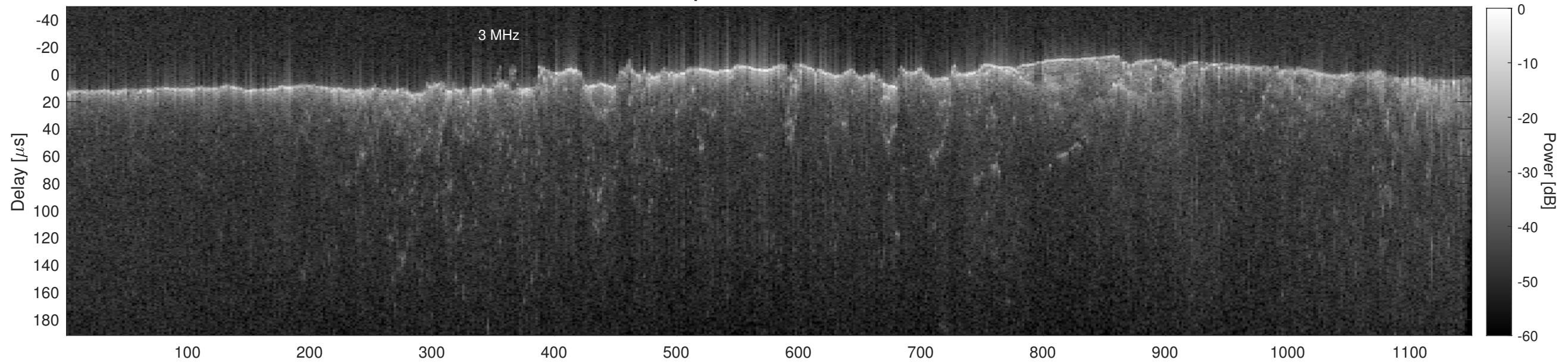
Orbit 17268, Cluttergram
