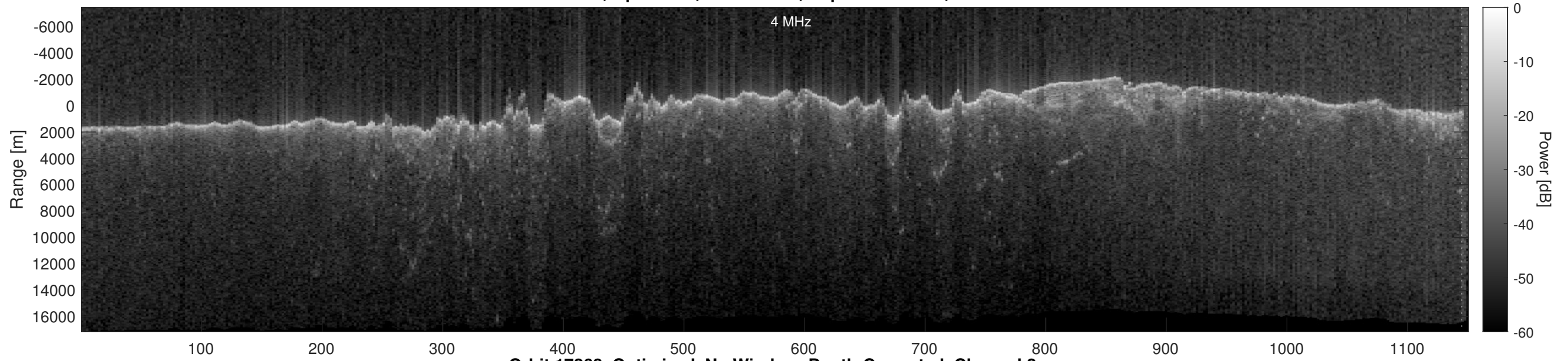
Orbit 17268, Optimized, No Window, Depth-Corrected, Channel 2
