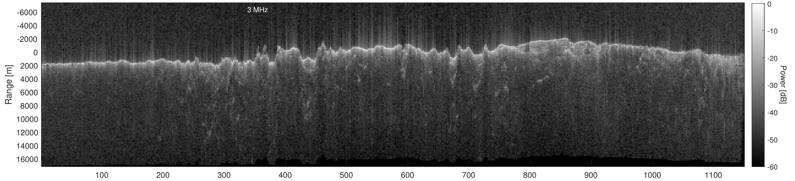
Orbit 17268, Depth-Corrected Cluttergram
