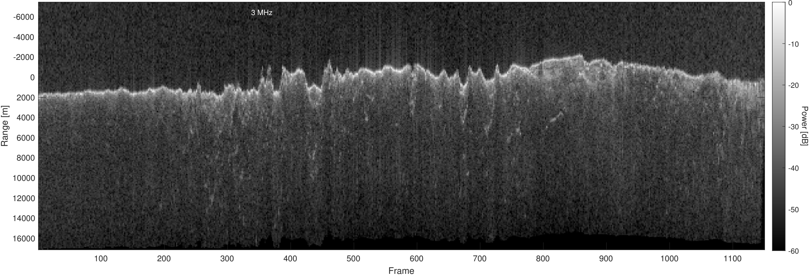
Orbit 17268, Optimized, Window, Depth-Corrected, Channel 2
