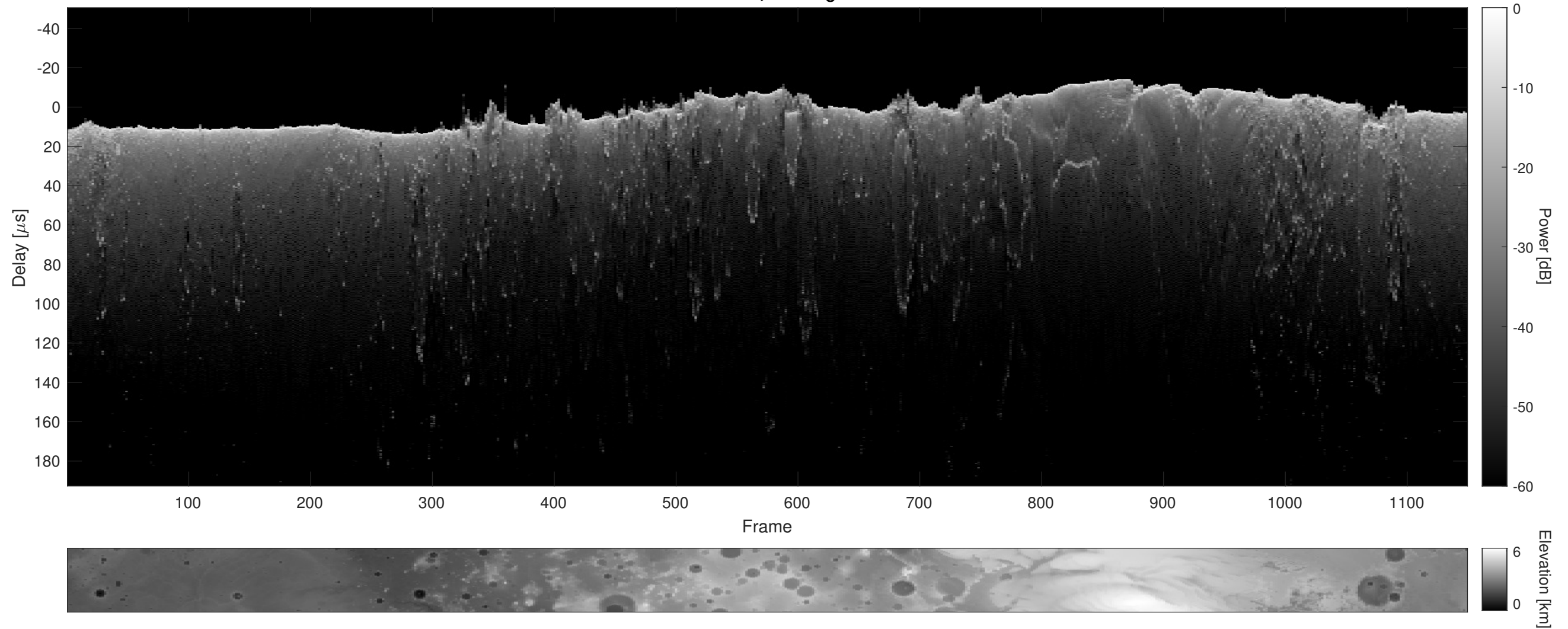
Orbit 17275, Cluttergram
