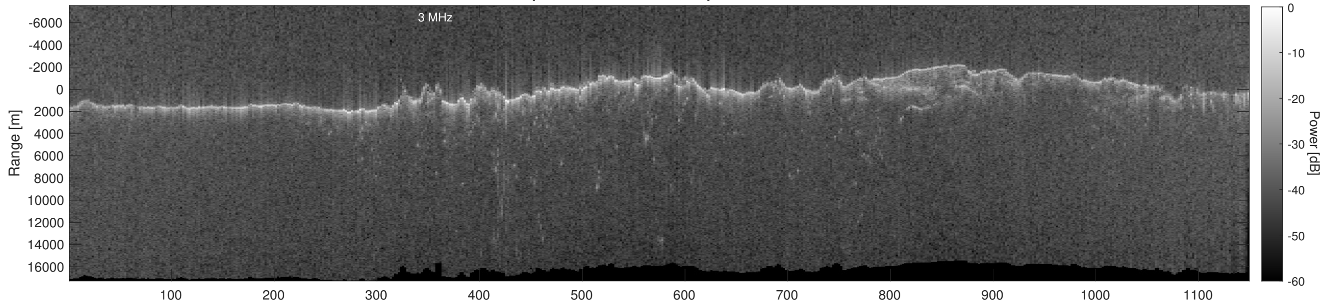
Orbit 17275, Depth-Corrected Cluttergram
