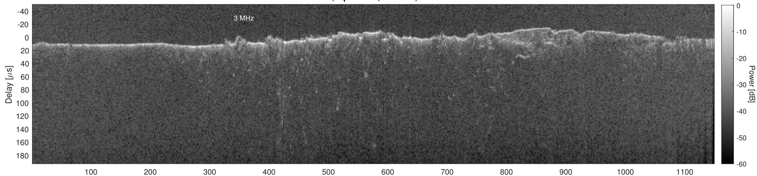
Orbit 17275, Cluttergram
