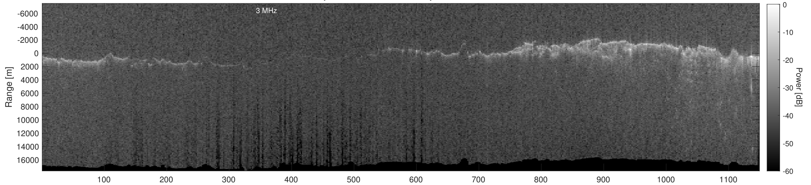
Orbit 17289, Depth-Corrected Cluttergram
