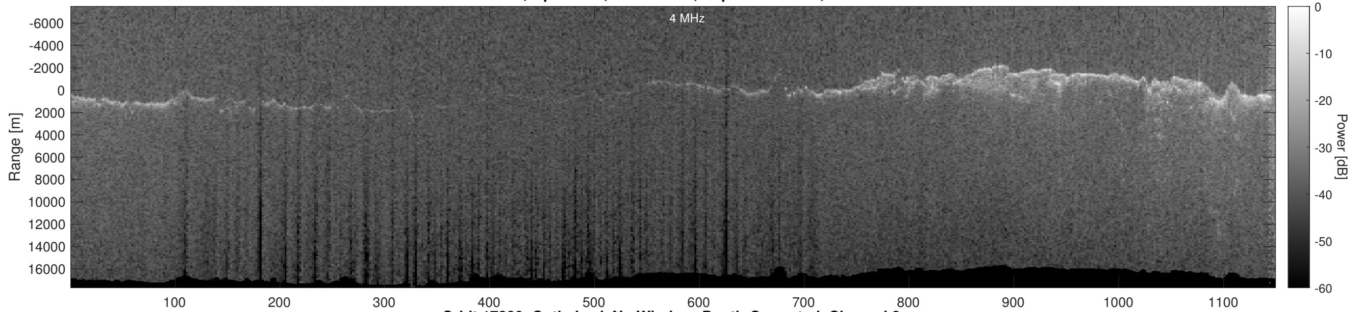
Orbit 17289, Optimized, No Window, Depth-Corrected, Channel 2
