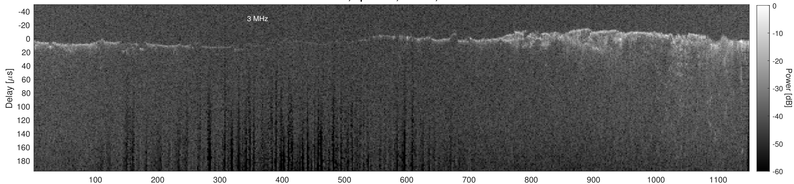
Orbit 17289, Cluttergram
