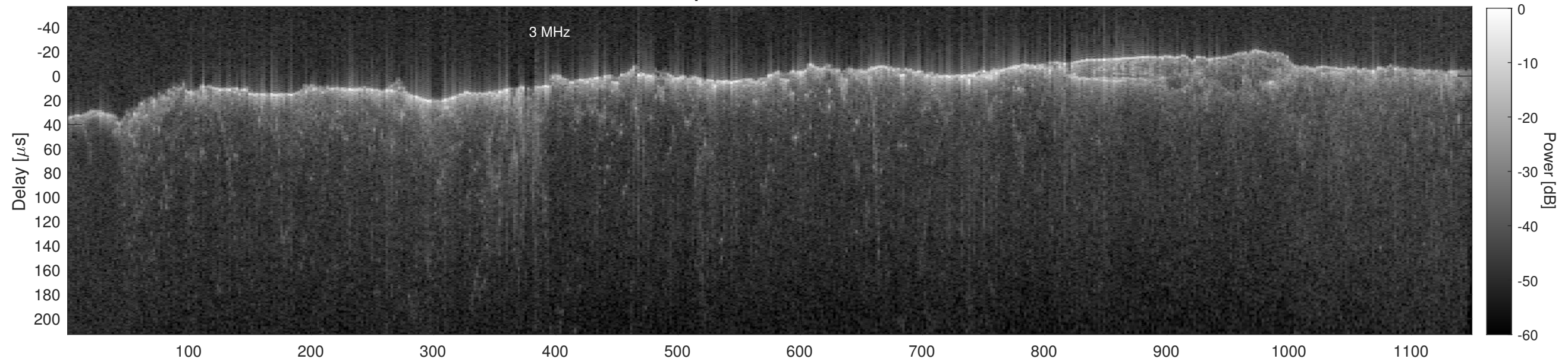
Orbit 17306, Cluttergram
