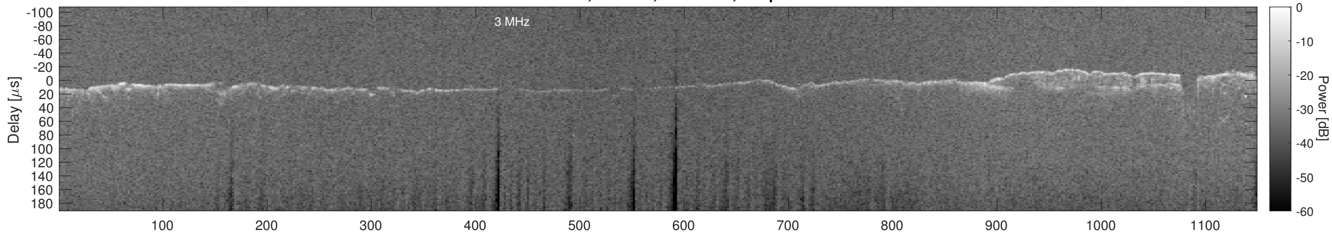
Orbit 17318, Window, Channel 2, Optimized
