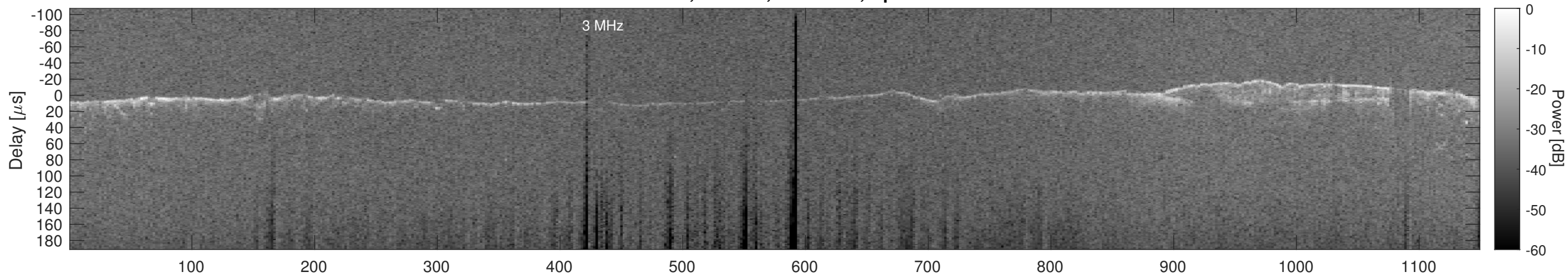
Orbit 17318, Cluttergram
