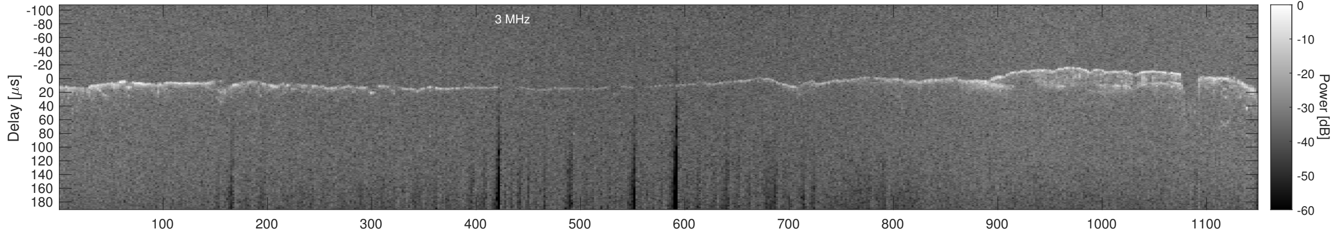
Orbit 17318, Window, Channel 2, Chapman
