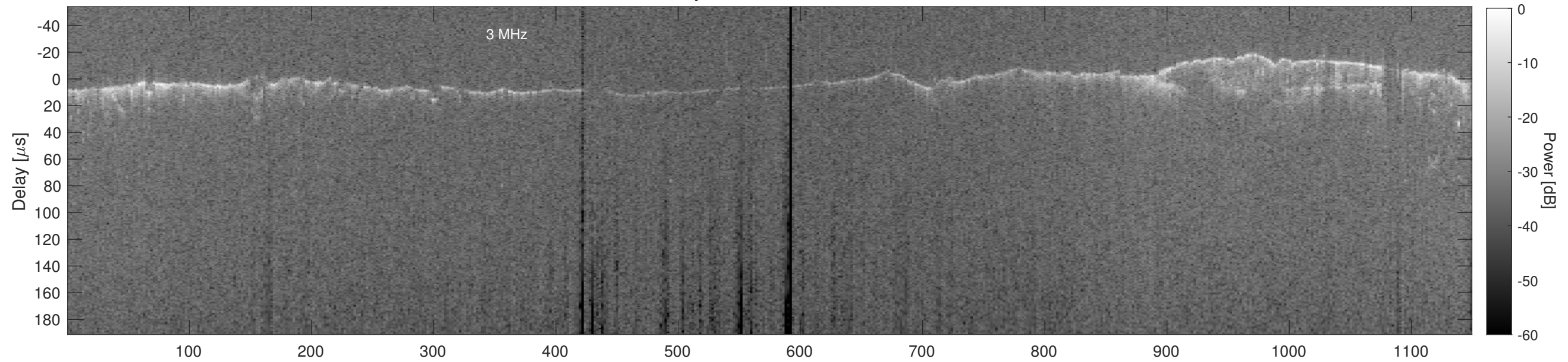
Orbit 17318, Cluttergram
