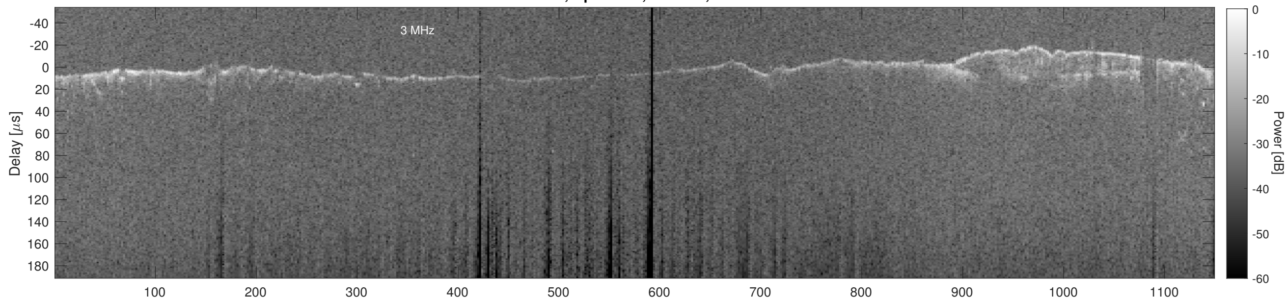
Orbit 17318, Cluttergram
