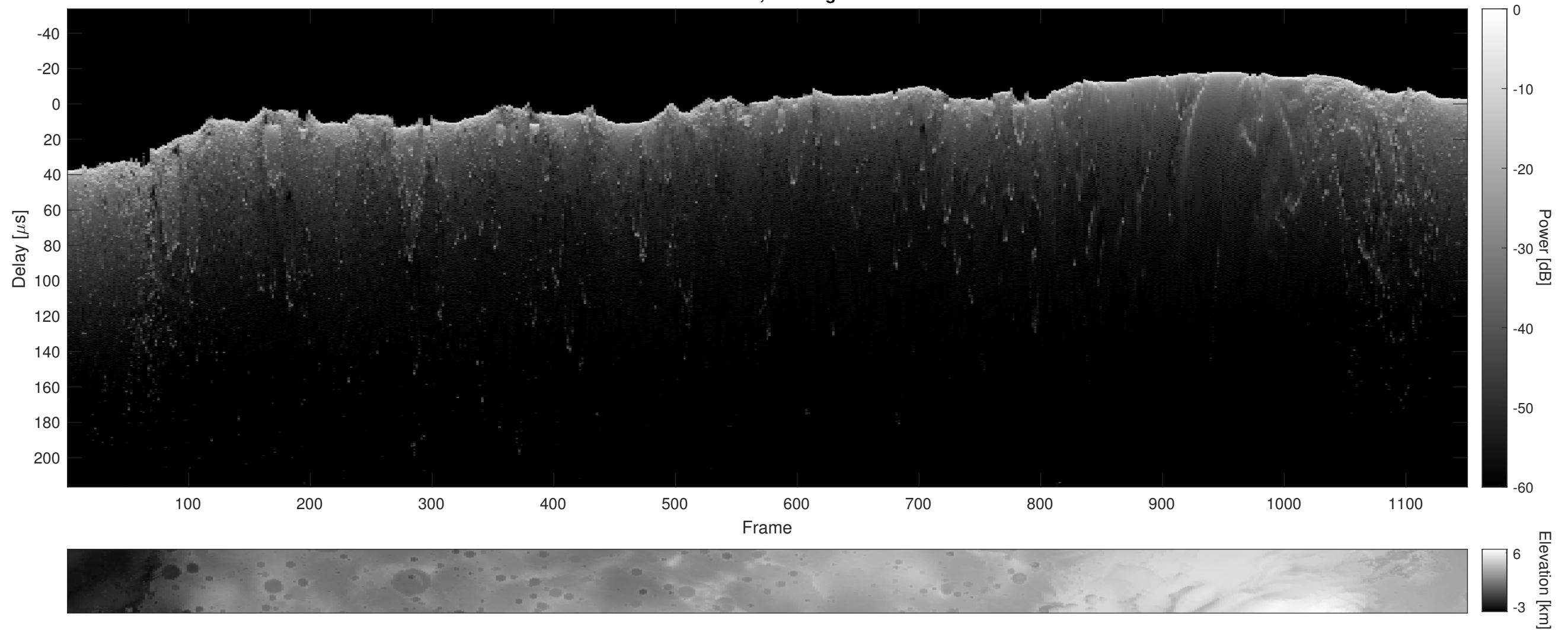
Orbit 17338, Cluttergram
