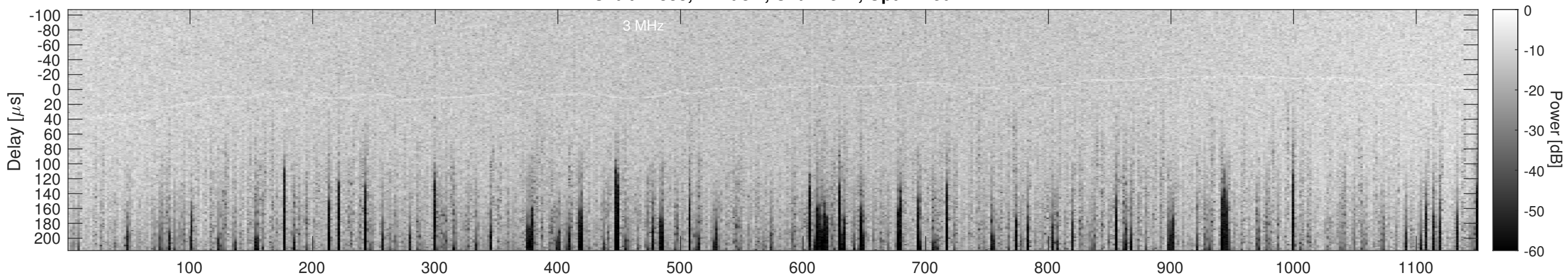
Orbit 17338, Cluttergram
