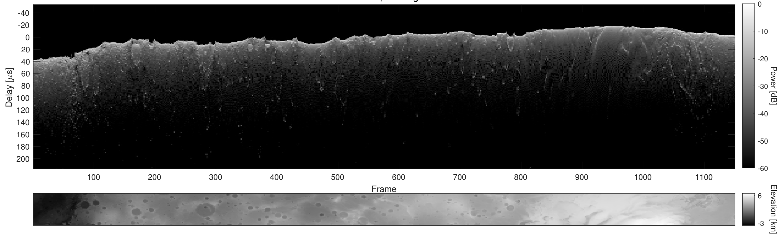
Orbit 17338, Cluttergram
