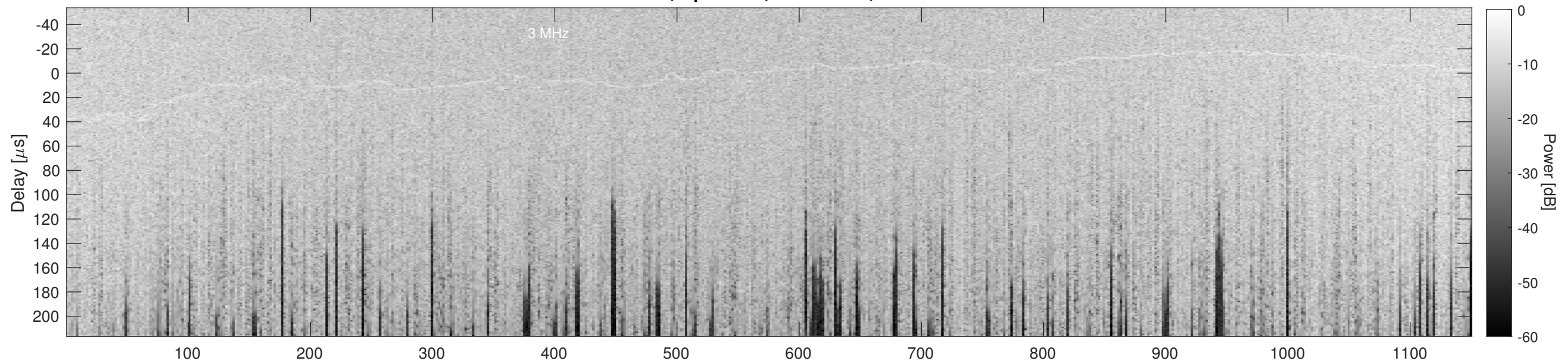
Orbit 17338, Cluttergram
