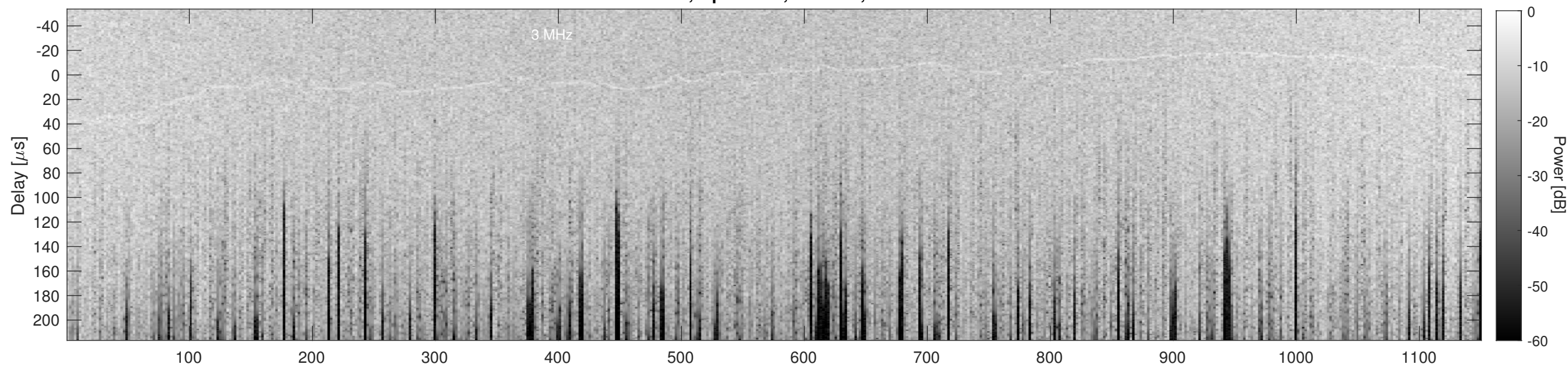
Orbit 17338, Cluttergram
