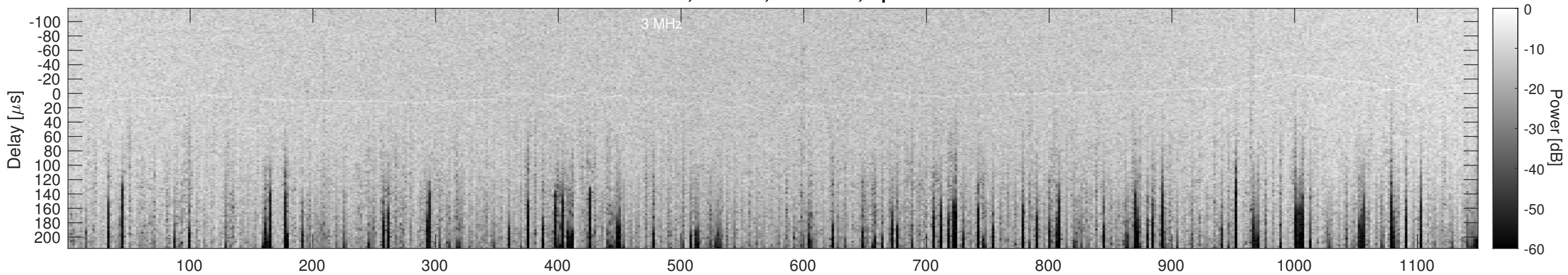
Orbit 17340, Cluttergram
