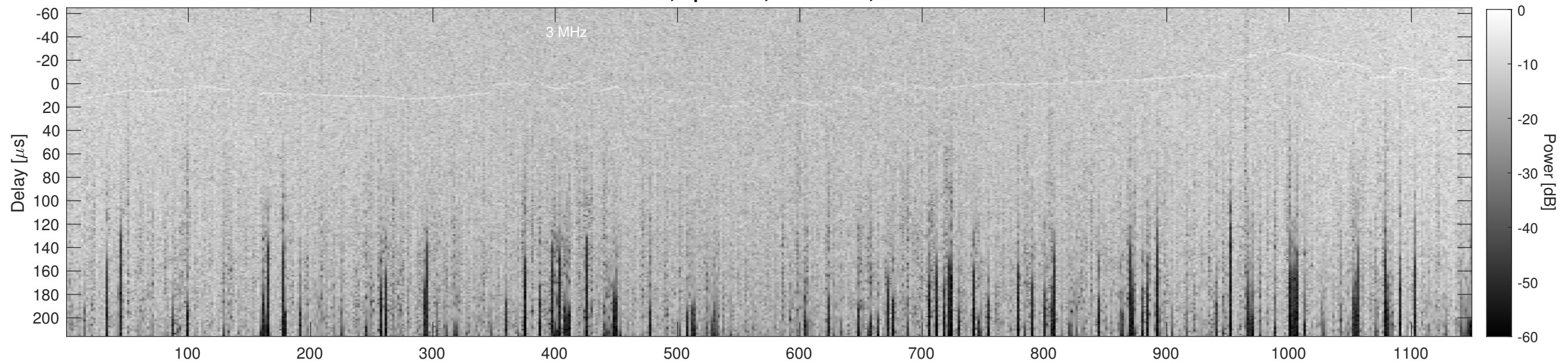
Orbit 17340, Cluttergram
