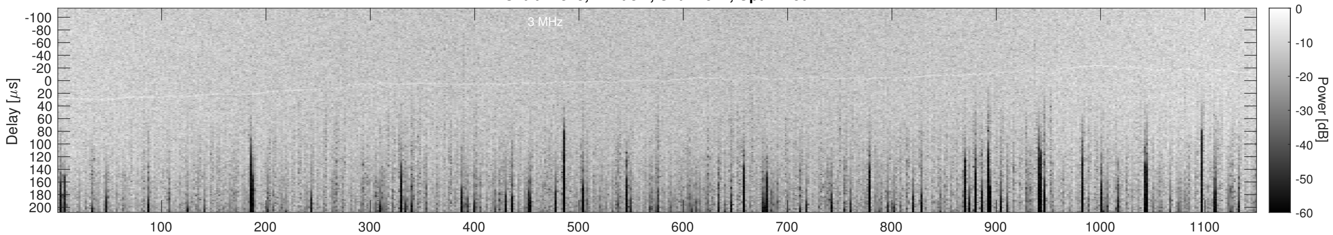
Orbit 17343, Cluttergram
