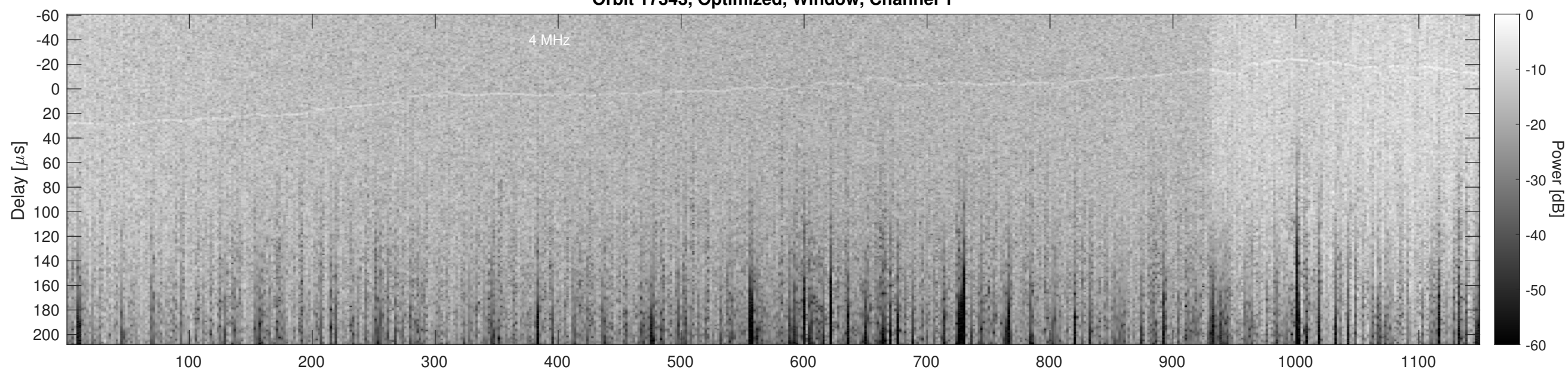
Orbit 17343, Optimized, Window, Channel 2
