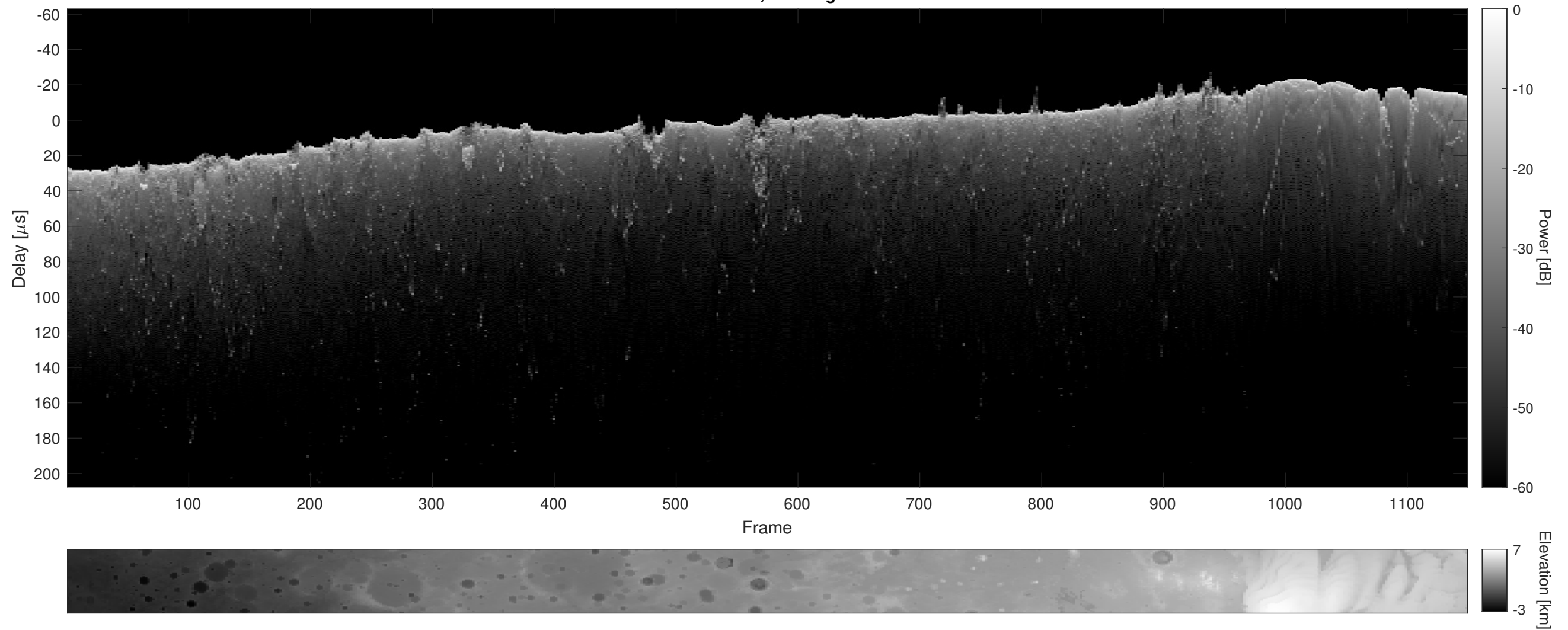
Orbit 17350, Cluttergram
