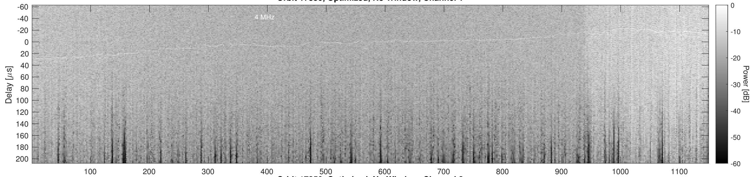
Orbit 17350, Optimized, No Window, Channel 2
