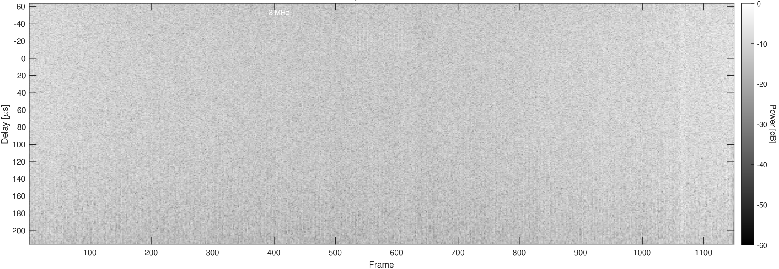
Orbit 17355, Chapman, No Window, Channel 2
