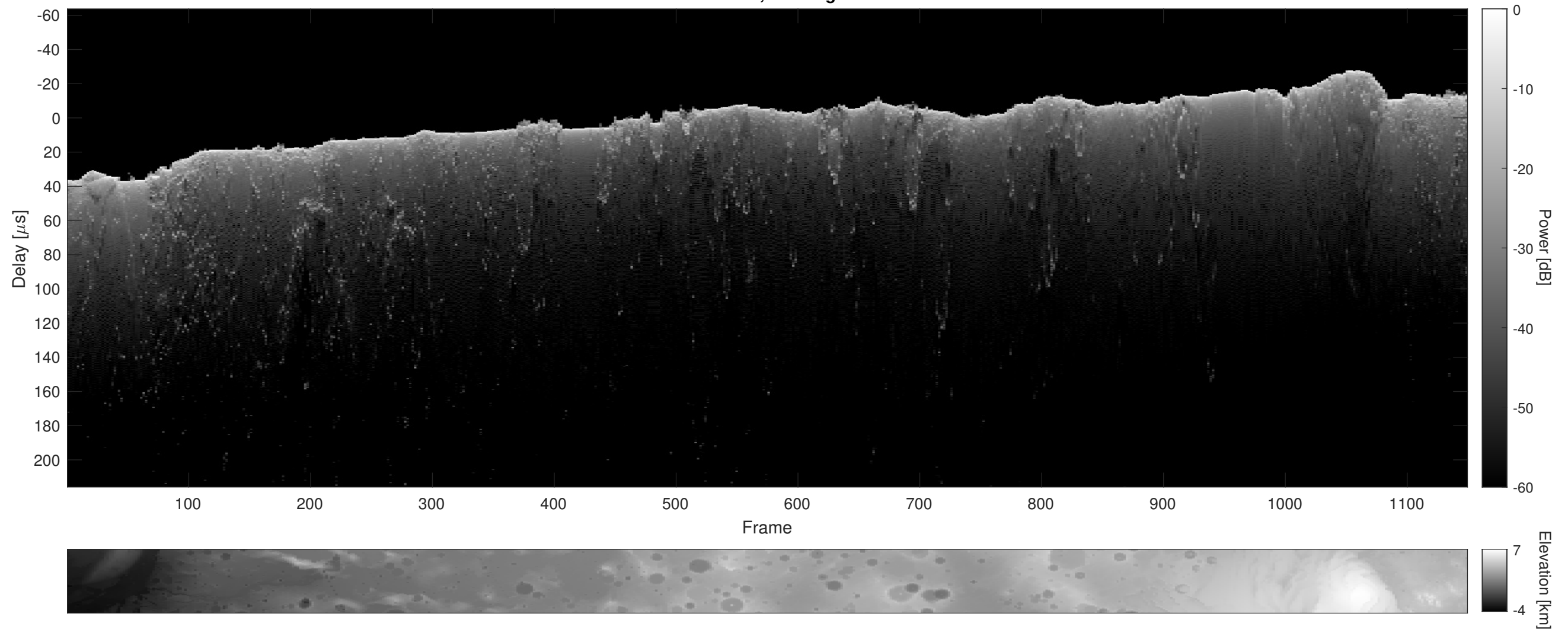
Orbit 17355, Cluttergram
