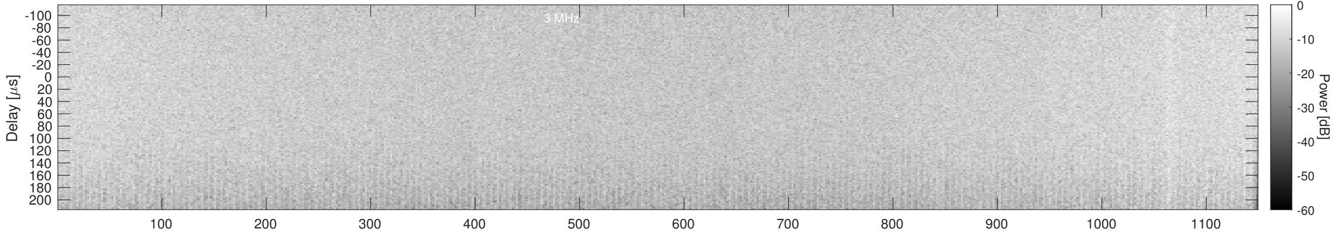
Orbit 17355, Window, Channel 2, Chapman
