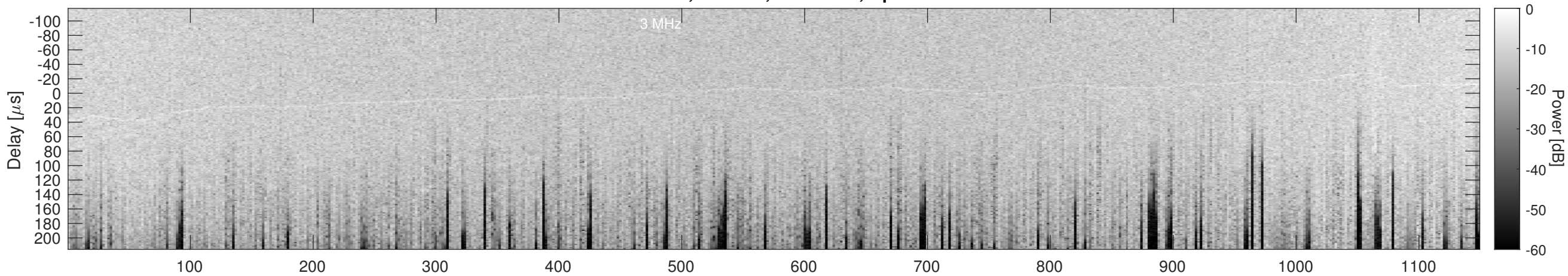
Orbit 17355, Cluttergram
