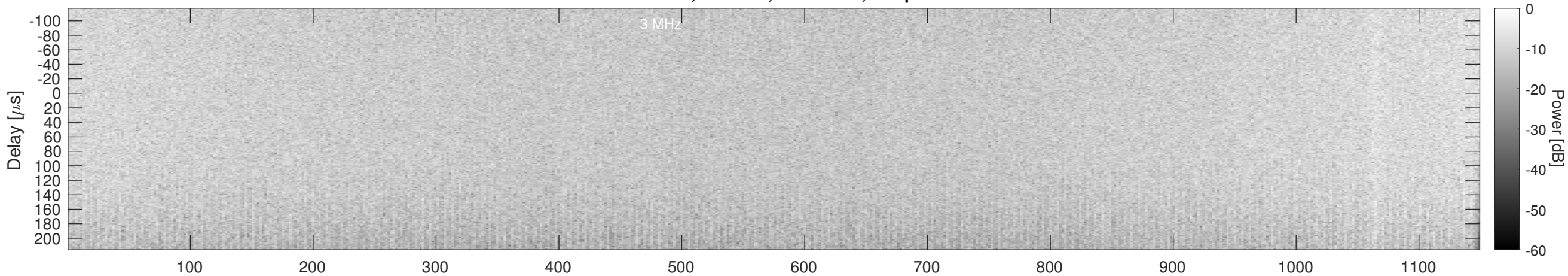
Orbit 17355, Window, Channel 2, Optimized
