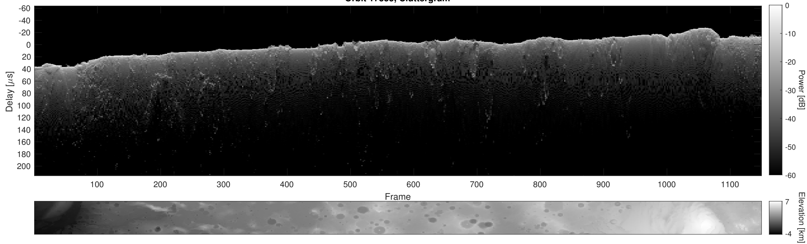
Orbit 17355, Cluttergram
