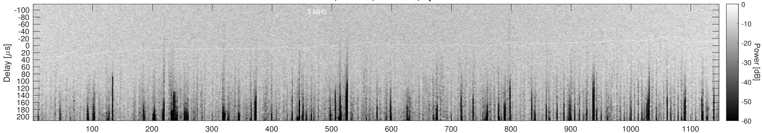
Orbit 17362, Cluttergram
