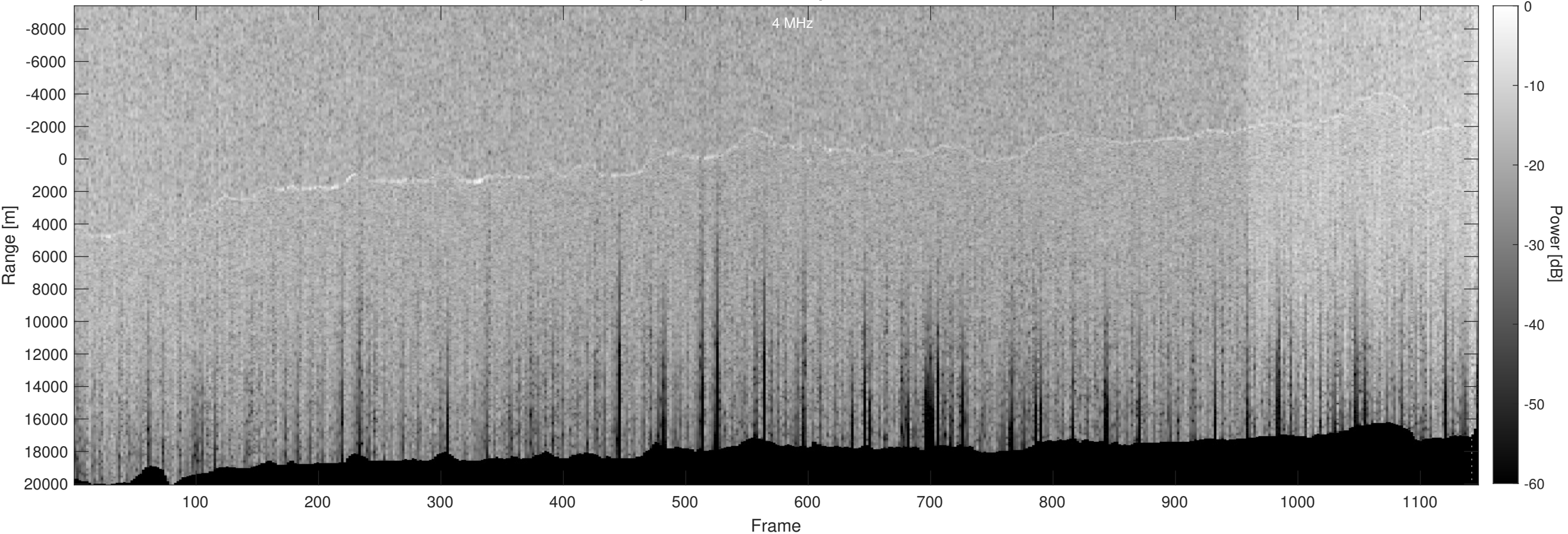
Orbit 17362, Optimized, Window, Depth-Corrected, Channel 2
