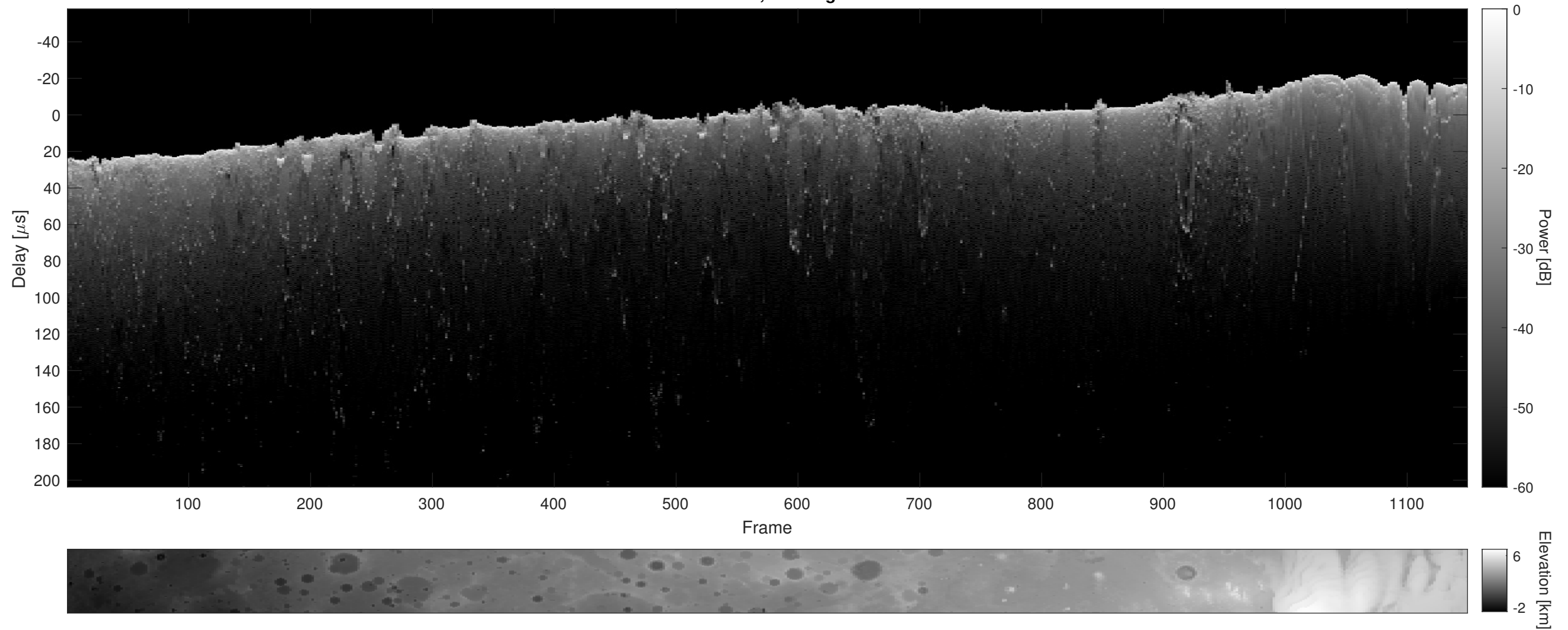
Orbit 17364, Cluttergram
