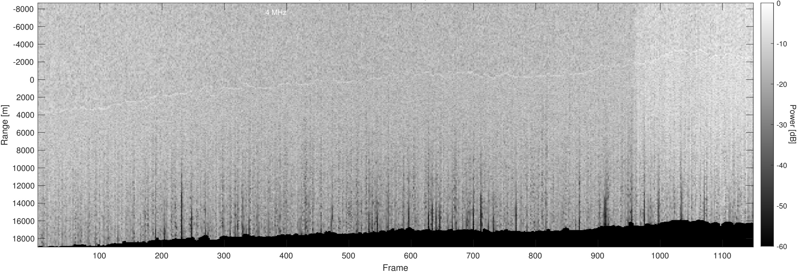
Orbit 17364, Optimized, No Window, Depth-Corrected, Channel 2
