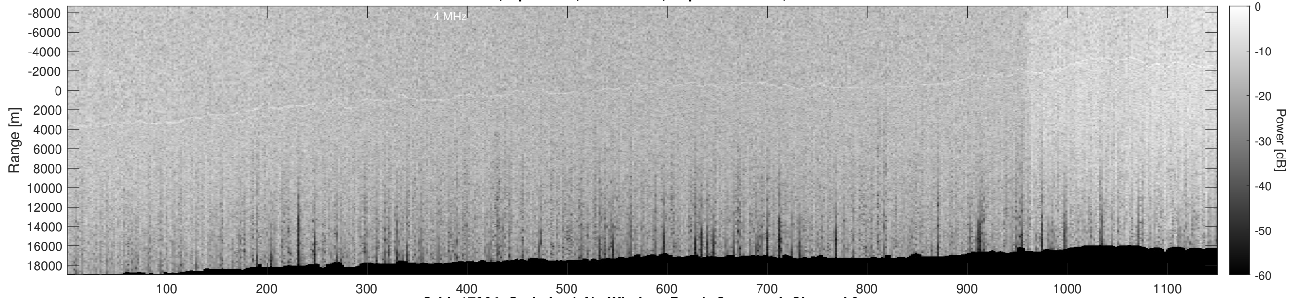
Orbit 17364, Optimized, No Window, Depth-Corrected, Channel 2
