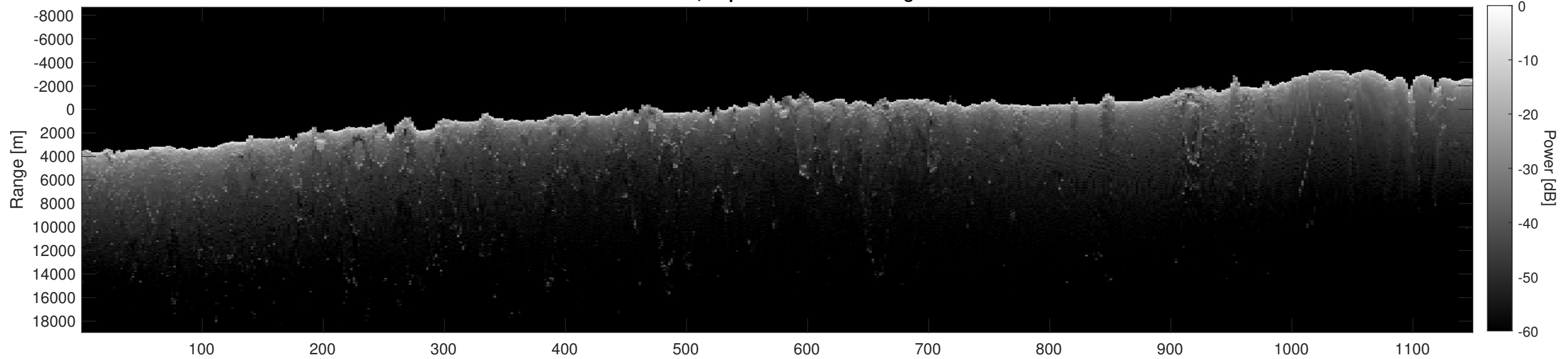
Orbit 17364, Depth-Corrected Cluttergram
