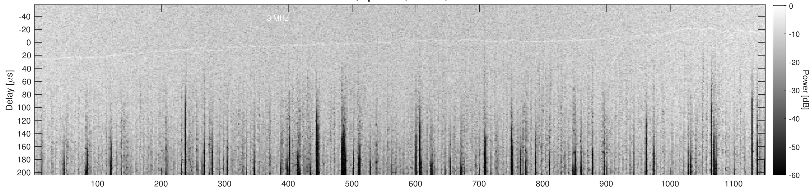
Orbit 17364, Cluttergram
