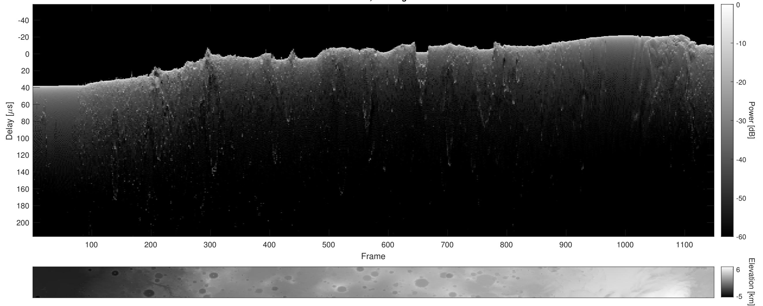
Orbit 17366, Cluttergram
