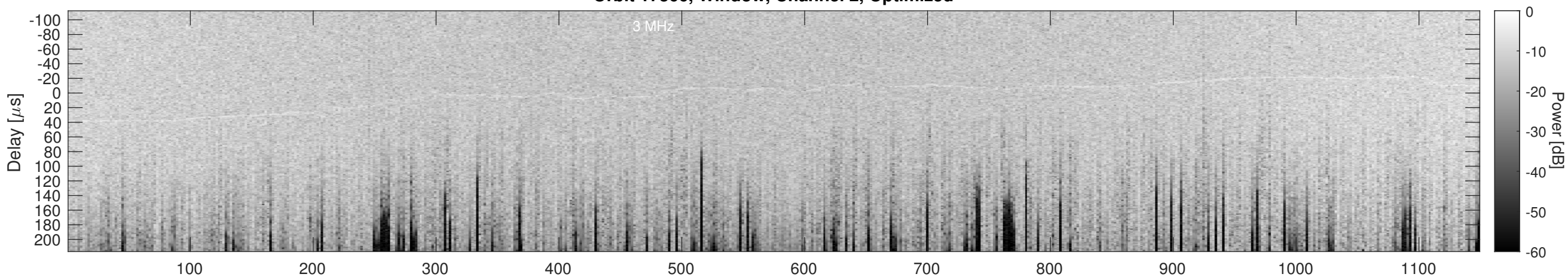
Orbit 17366, Cluttergram
