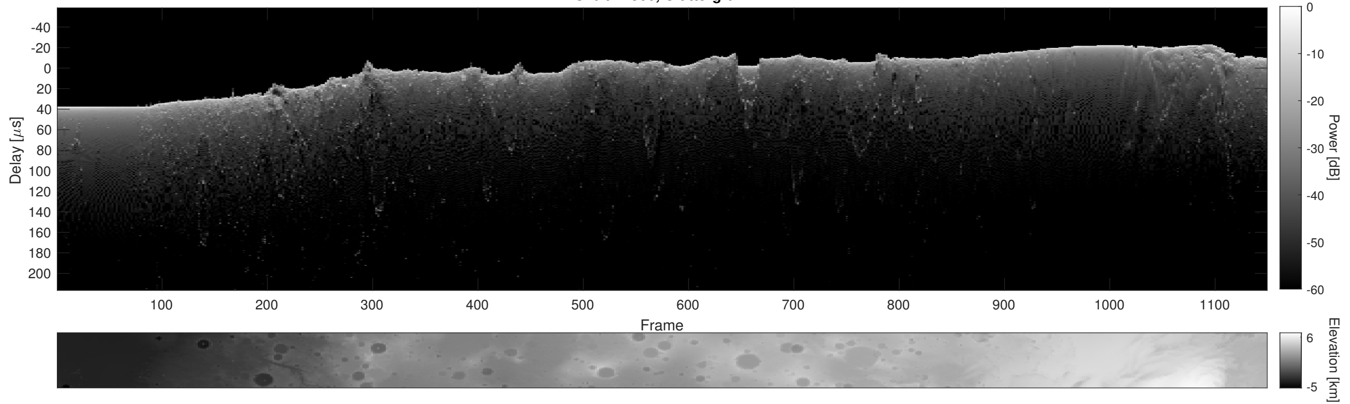
Orbit 17366, Cluttergram
