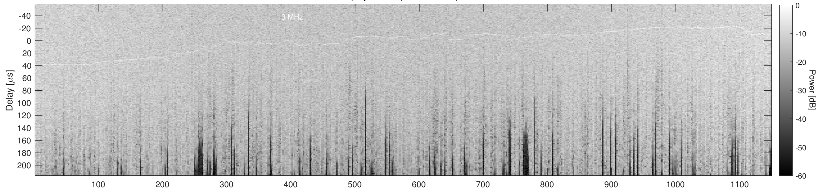
Orbit 17366, Cluttergram
