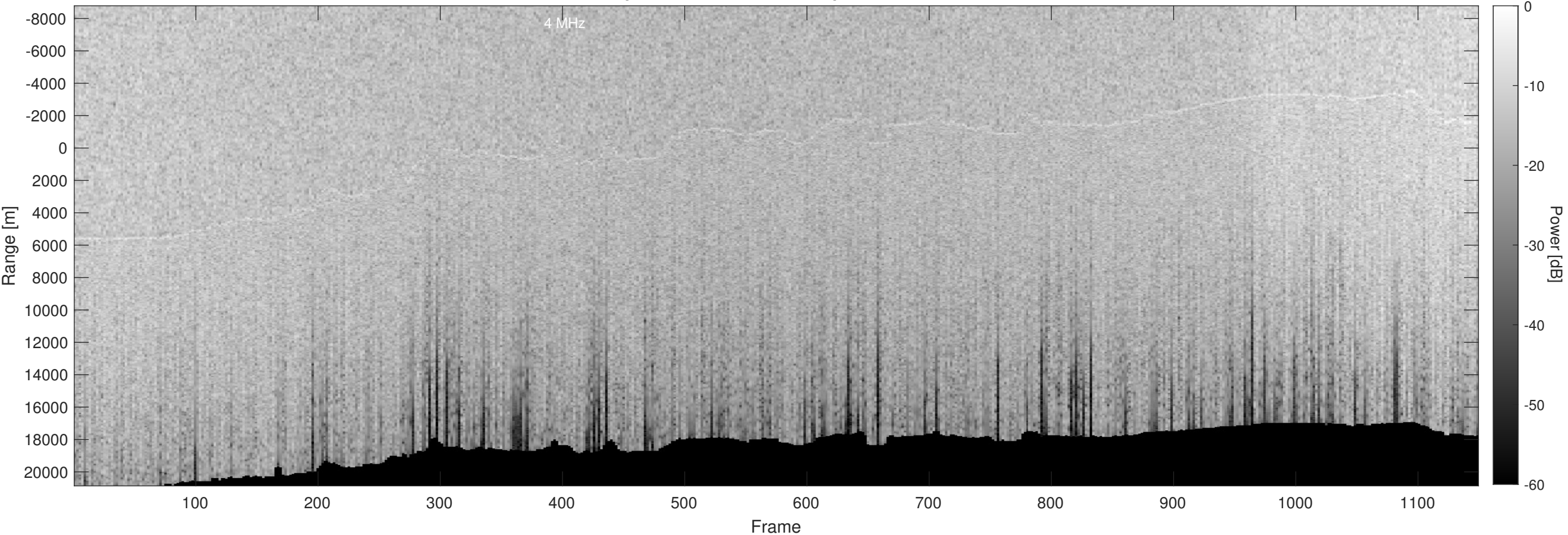
Orbit 17366, Optimized, No Window, Depth-Corrected, Channel 2
