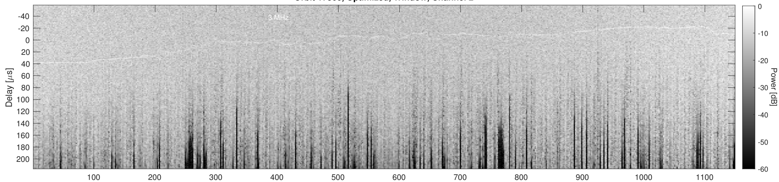
Orbit 17366, Cluttergram
