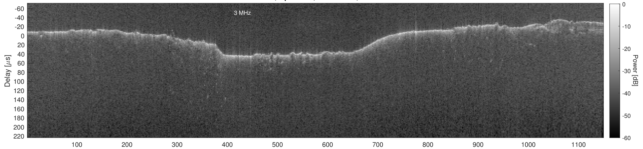
Orbit 17381, Cluttergram
