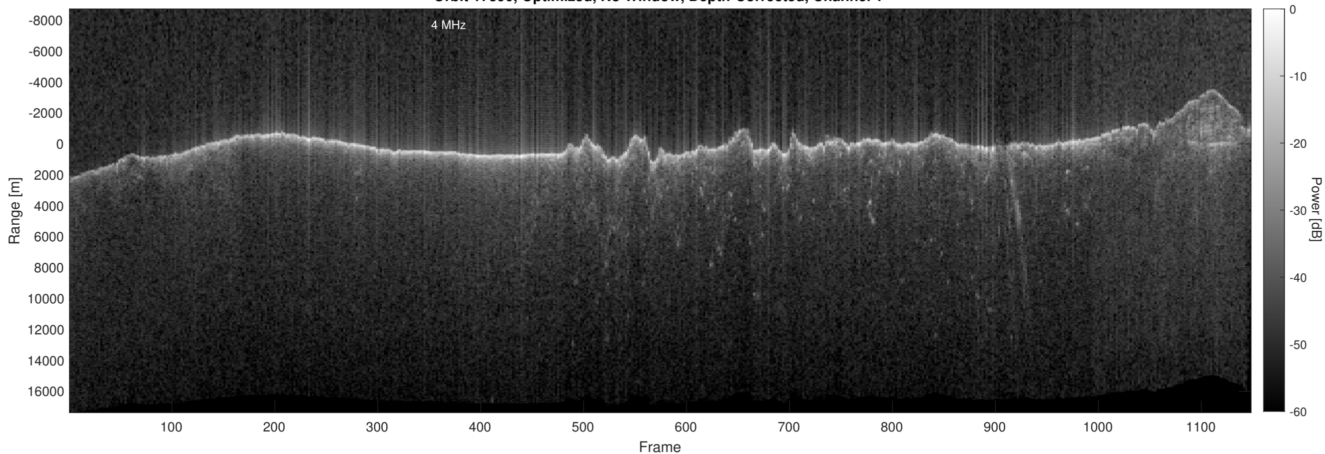
Orbit 17390, Optimized, No Window, Depth-Corrected, Channel 2
