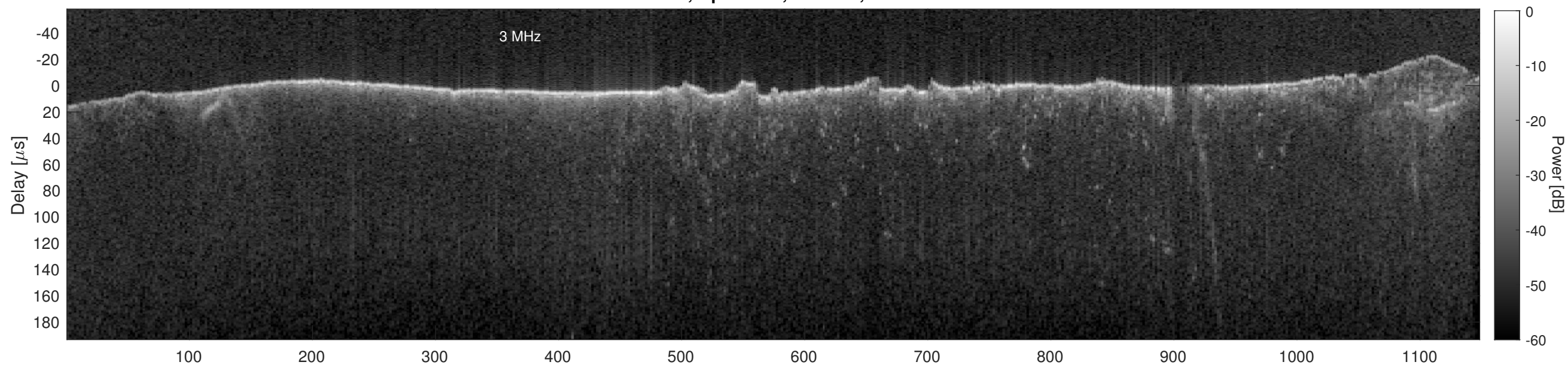
Orbit 17390, Cluttergram
