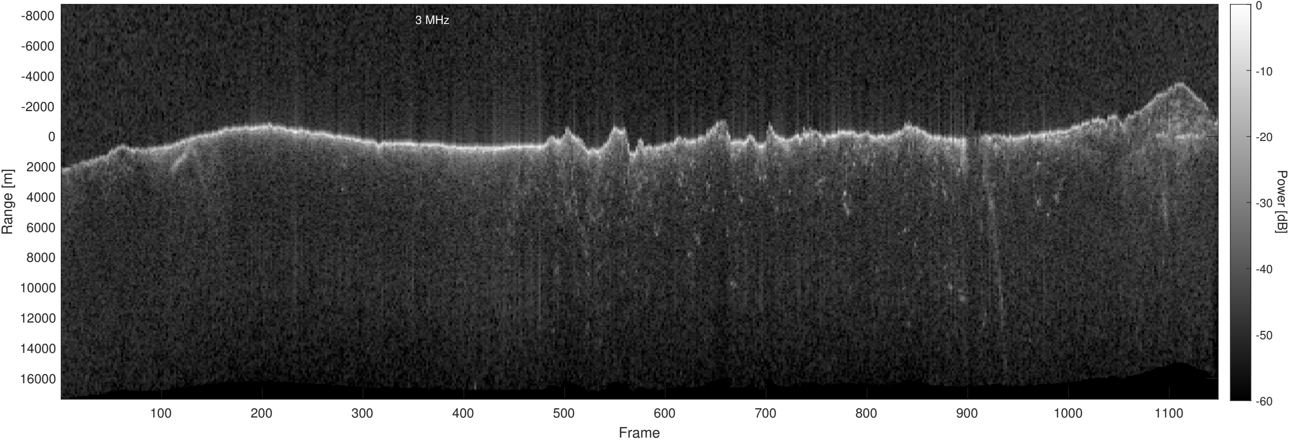
Orbit 17390, Optimized, Window, Depth-Corrected, Channel 2
