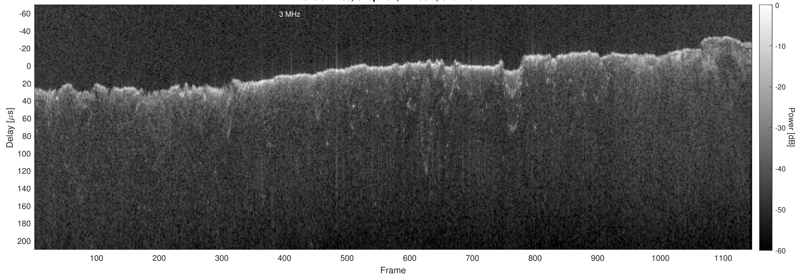
Orbit 17403, Chapman, Window, Channel 2
