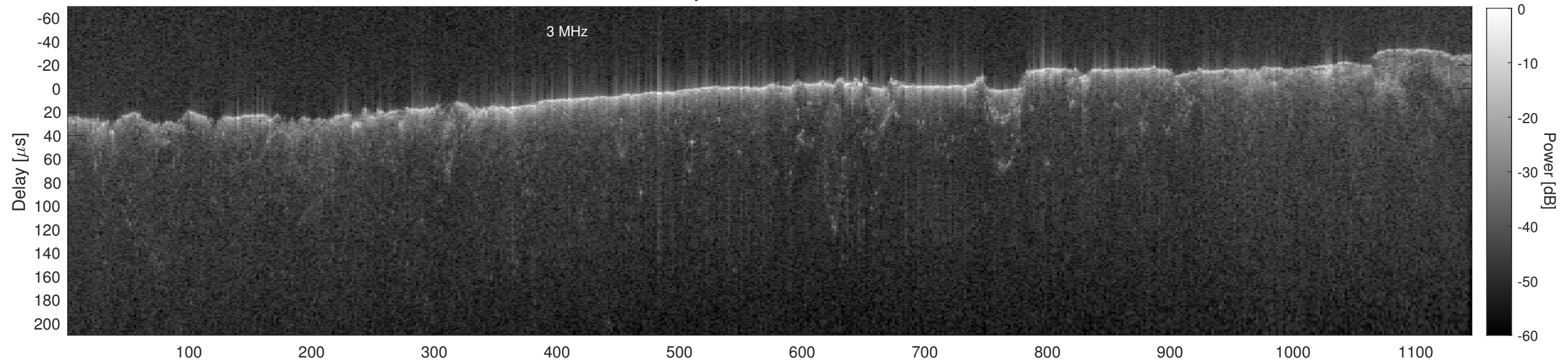
Orbit 17403, Cluttergram
