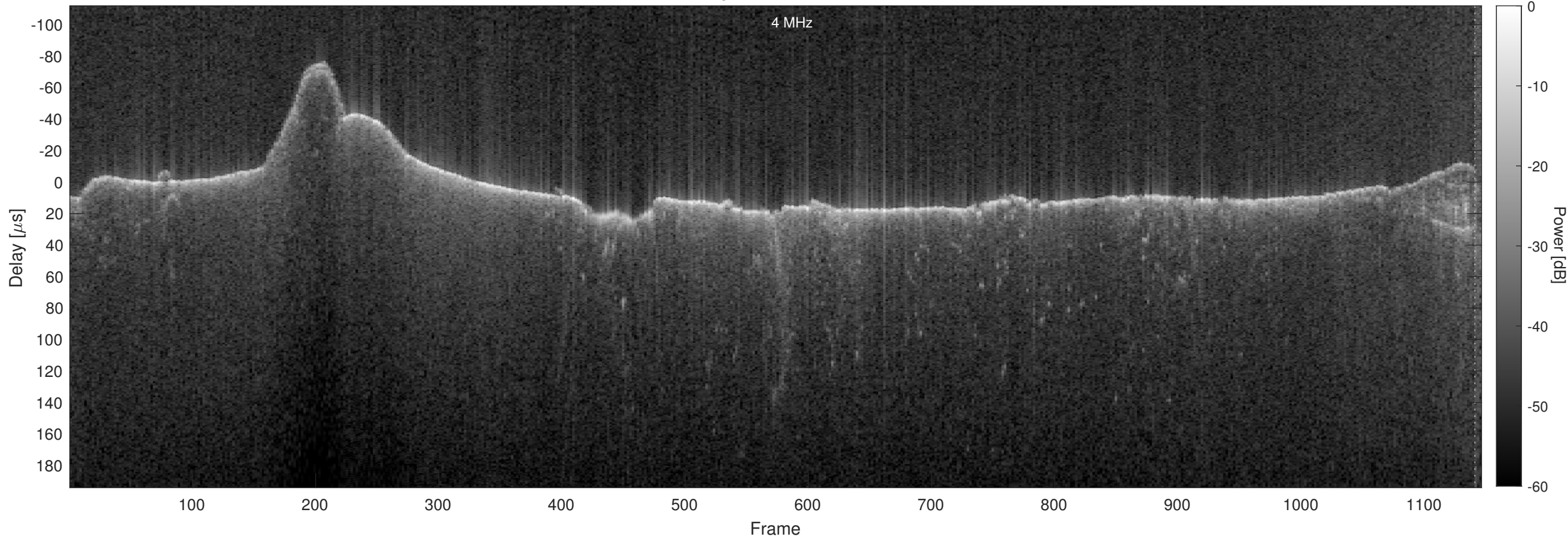
Orbit 17404, Chapman, No Window, Channel 2
