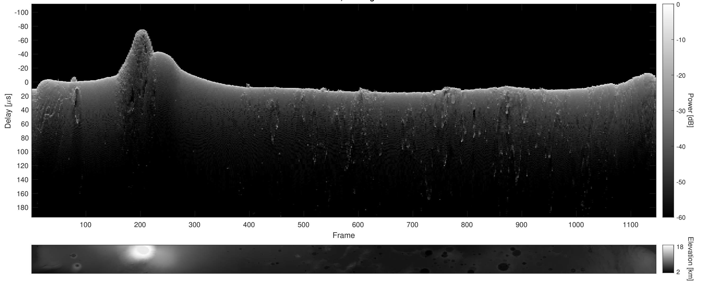
Orbit 17404, Cluttergram
