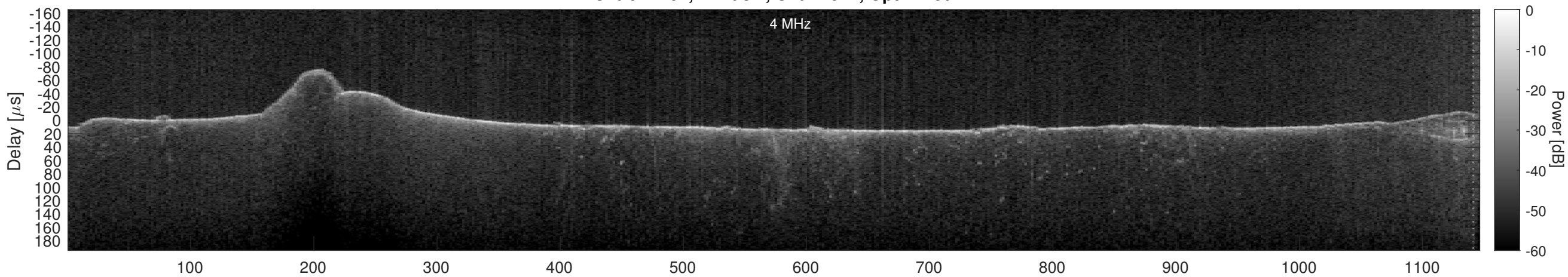
Orbit 17404, Cluttergram
