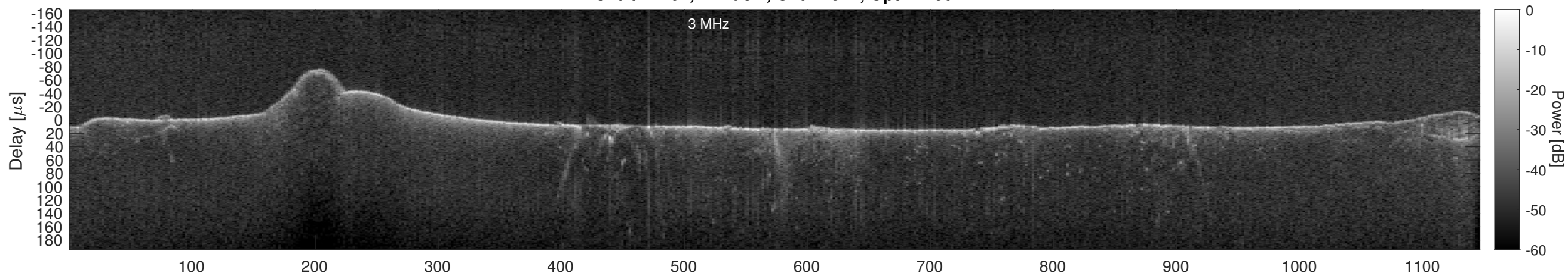
Orbit 17404, Cluttergram
