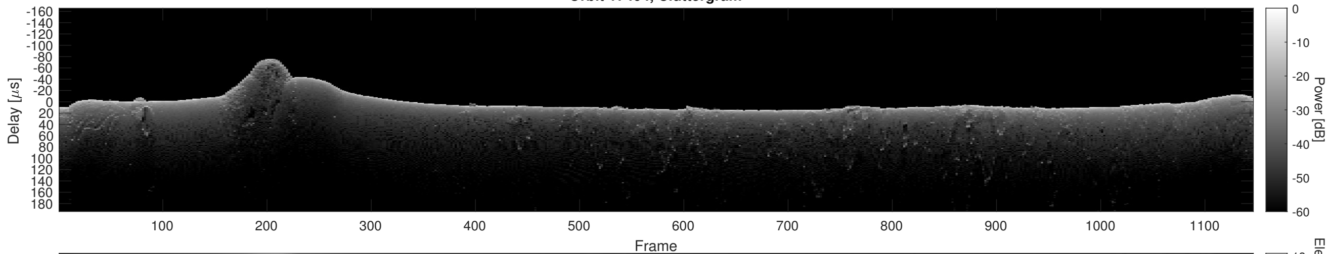
Orbit 17404, Cluttergram
