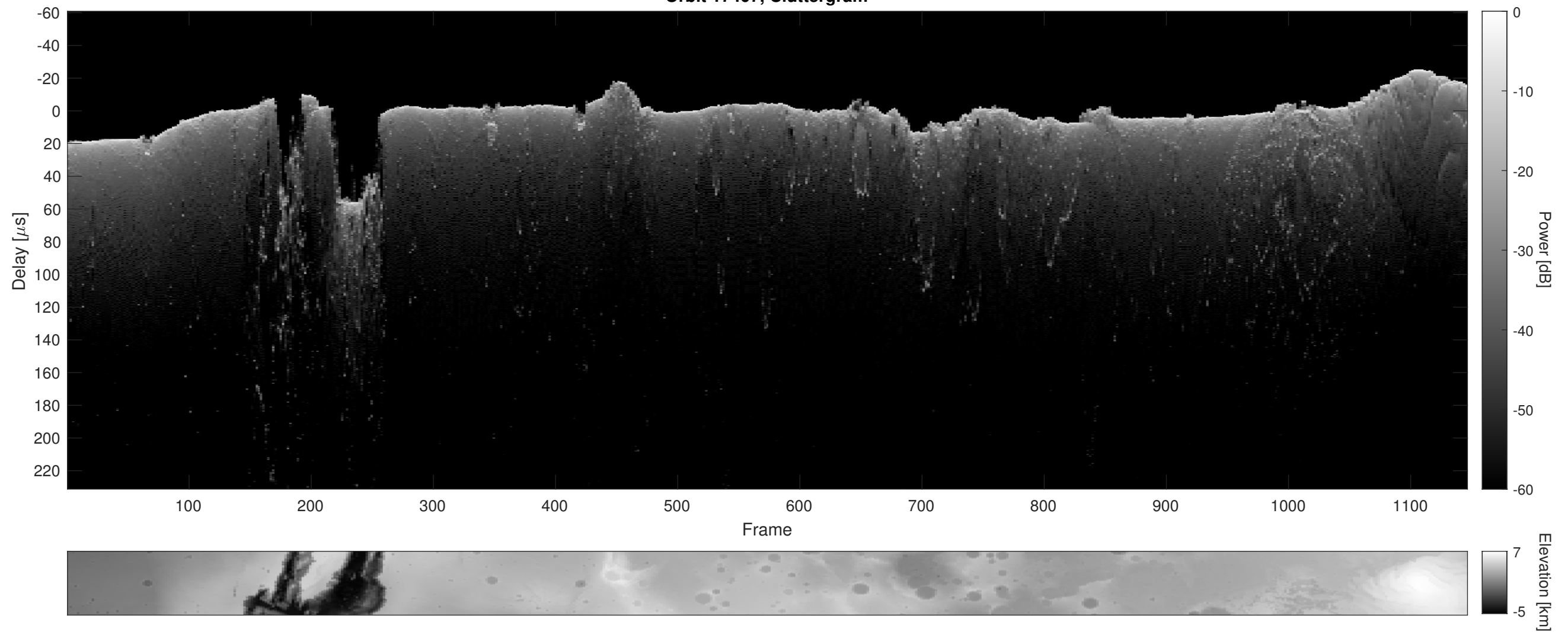
Orbit 17407, Cluttergram
