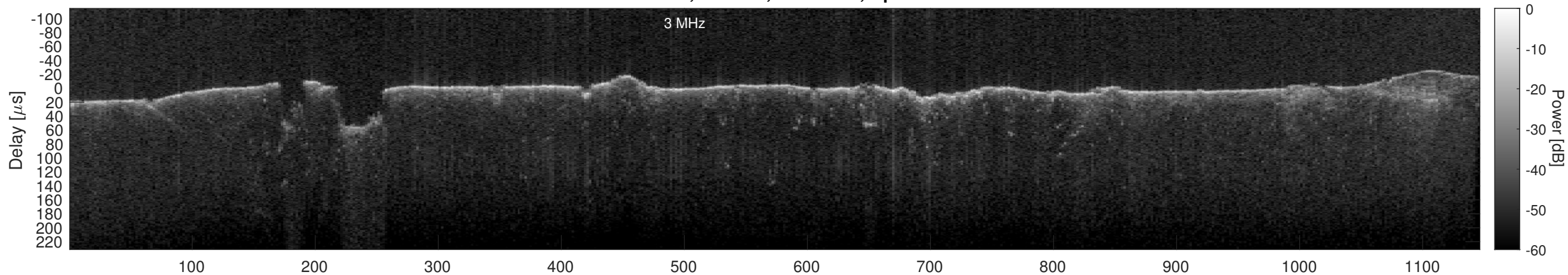
Orbit 17407, Cluttergram
