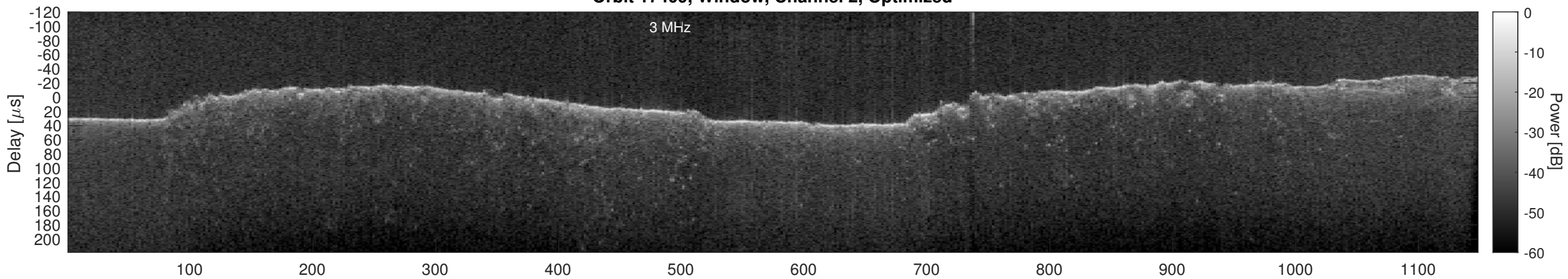
Orbit 17409, Cluttergram
